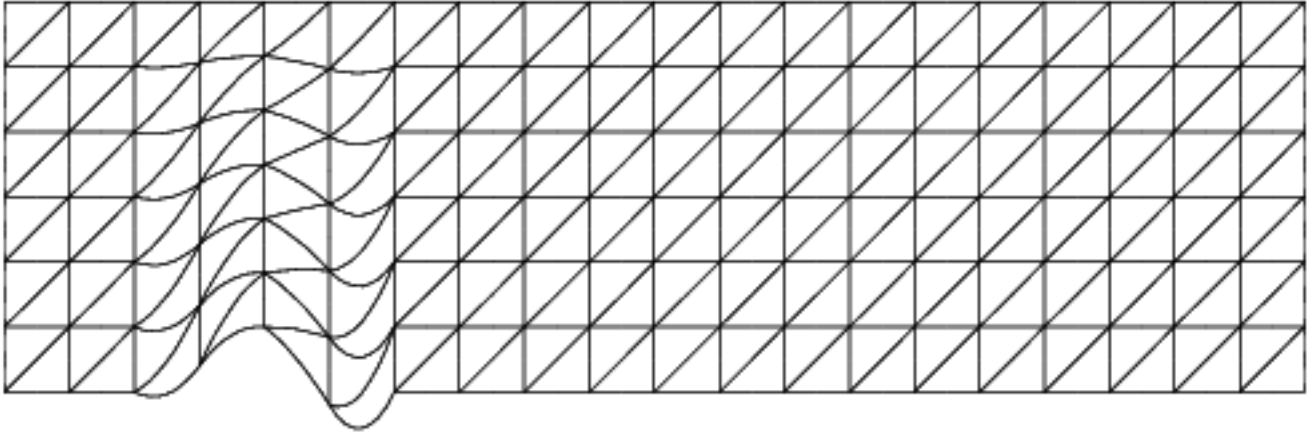
Figure 4.3: Decomposition of a flow region into elements. These elements are built from the nodes shown in Figure ??.
