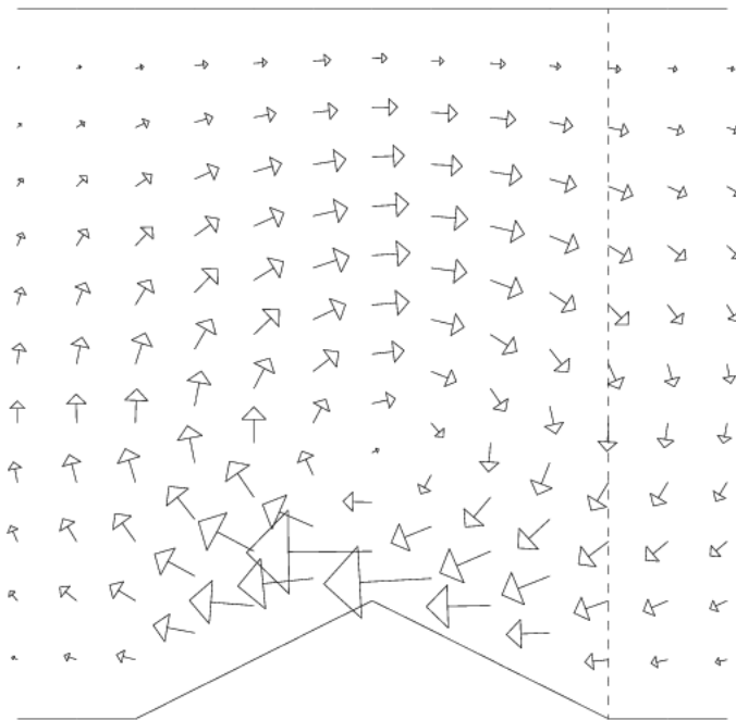
Figure 8.3: Adjusted finite difference \alpha -sensitivity nodal values.
