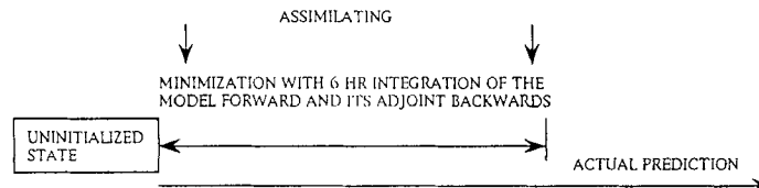
Figure 5. A schematic view of the assimilation-forecast cycle.
