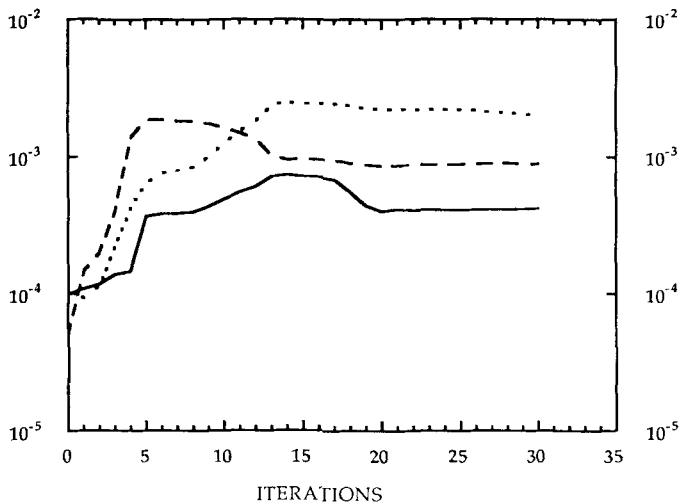
Figure 2. Variation of the nudging coefficients, G_{inps} (—), G_D (---) and G_\zeta (.), with the number of iterations. Both the initial conditions and the nudging coefficients G_{inps} , G_D and G_\zeta serve as control variables. The length of the assimilation window is 6 hours.
