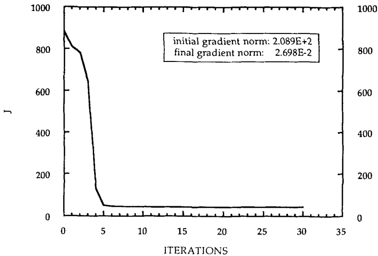
Figure 1. Variation of the cost function, \mathcal{J} , with the number of iterations. Both the initial conditions and the nudging coefficients, G_{inps} , G_D and G_\zeta , serve as control variables. The norms of initial gradient, \|g_0\| , and final gradient, \|g\| , (30 iterations) are also given. The length of the assimilation window is 6 hours.
